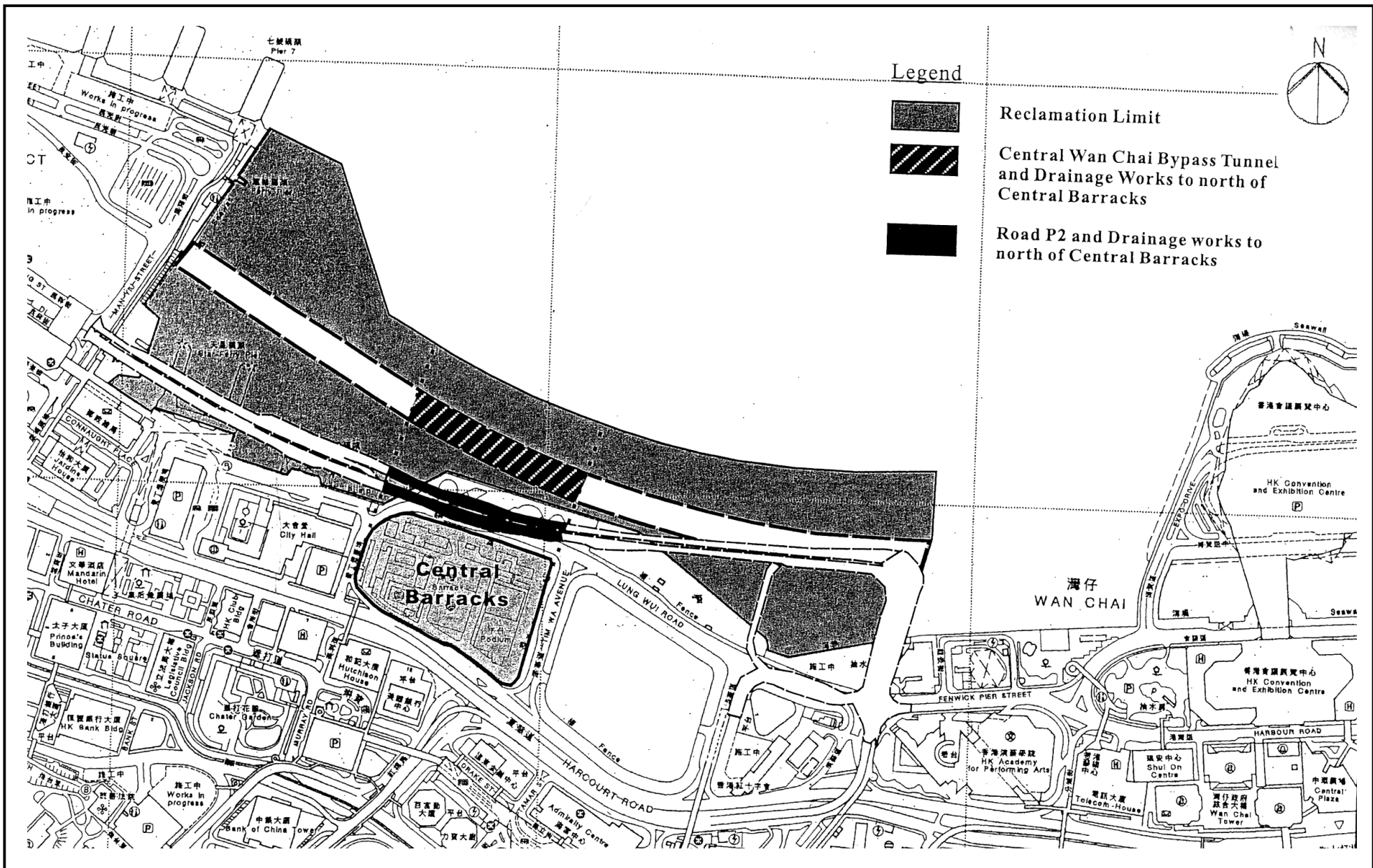
Figure 8: Locations of Road P2 and Drainage Works to North of Central Barracks Note: Locations of Road P2 and Drainage Works to North of Central Barracks Modified from Figure 4.2 of Volume 1 of the EIA Report
